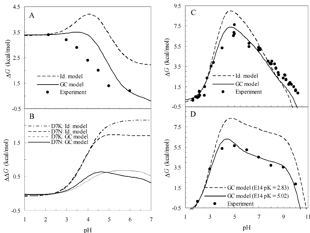
FIGURE 5: pH dependence of the unfolding free energy for (A) Fnf3(10), (B) its Asp7Lys and Asp7Asn mutants, (C) ribonuclease Sa, and (D) its 5K mutant. Symbols are experimental results (64, 73), and curves are predictions by the Gaussian chain model (GC model) or an idealized model (Id. model) neglecting residual charge–charge interactions. In panel B, the reference is the unfolding free energy at pH 2.4.
