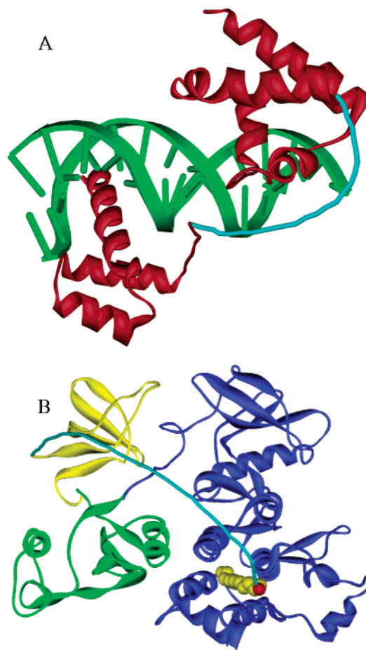
FIGURE 2: Flexible linkers (A) between the POU-specific domains and homeodomains of DNA-binding protein Oct-1 POU (112) and (B) between the SH3 domain (yellow) and a myristoyl group bound to the kinase domain (blue) of the tyrosine kinase c-Abl (120). The linkers are missing in the X-ray structures and are shown for illustration in cyan. C-Abl also has relatively rigid linkers between the SH3 domain and the SH2 domain (in green) and between the SH2 domain and the kinase domain.
